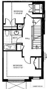
Second Floor
