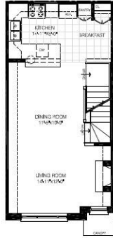
Main Floor
